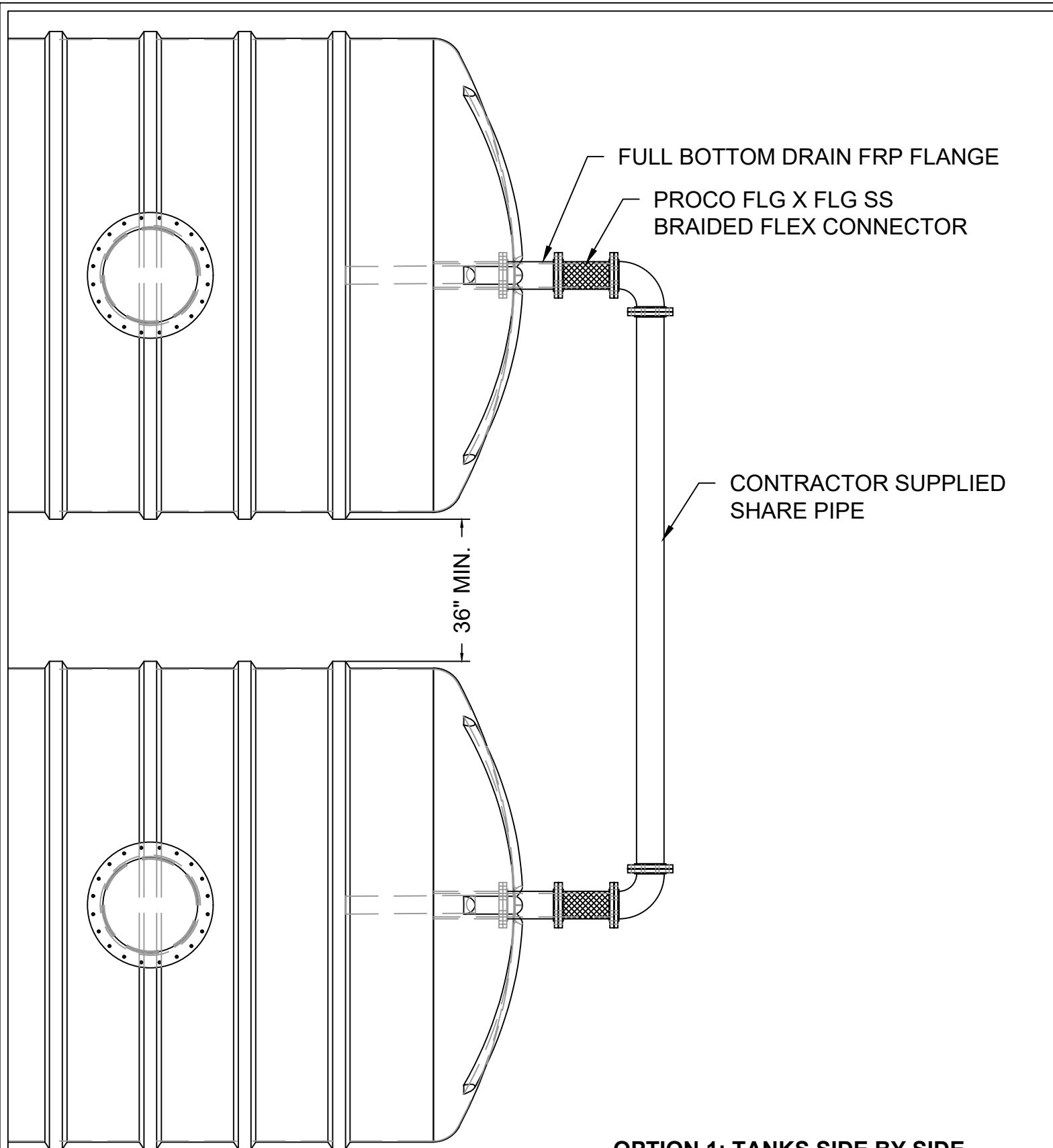
OPTION 1: TANKS SIDE BY SIDE TOP VIEW
