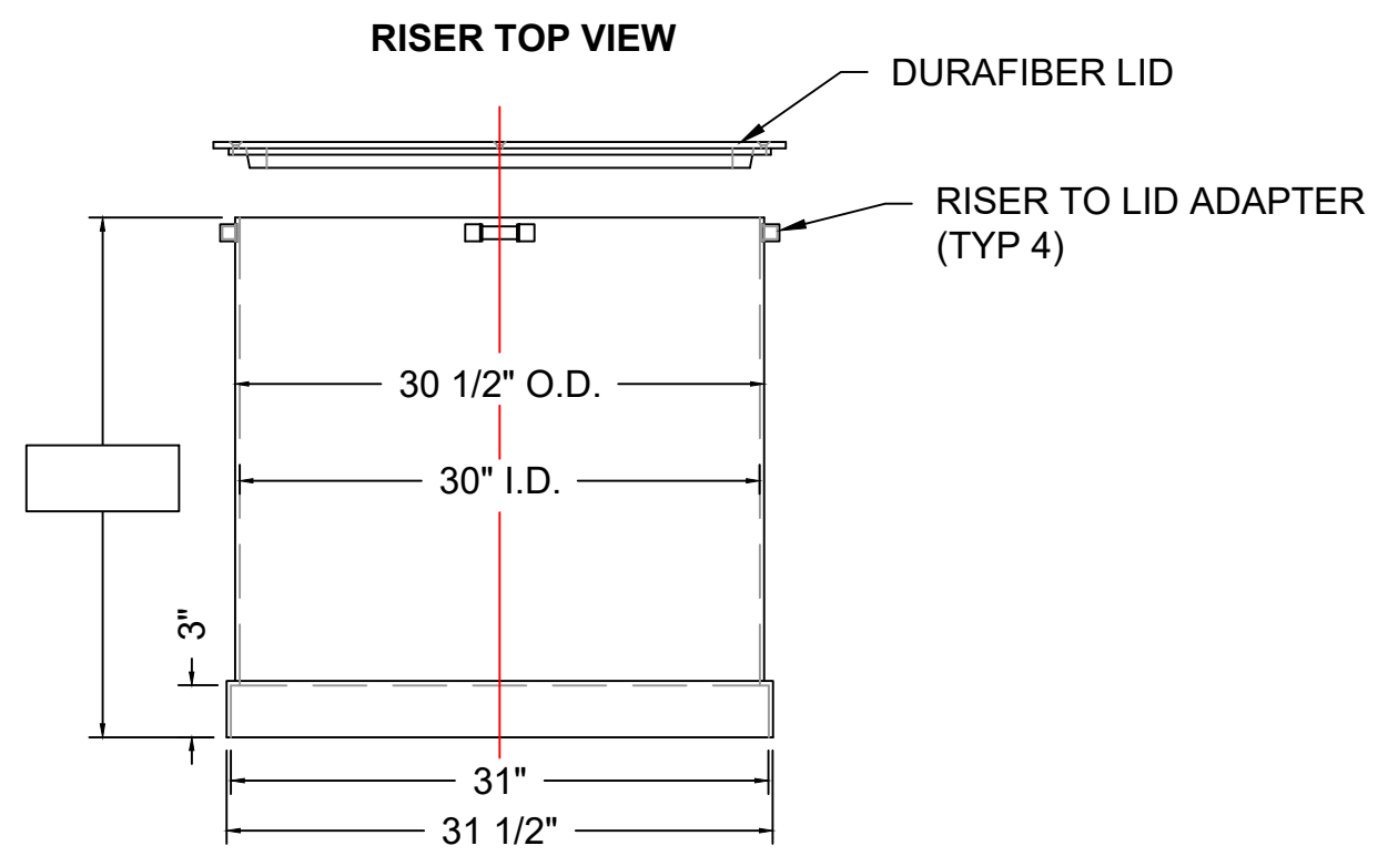
FRONT VIEW
